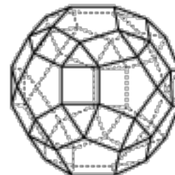
Rhombicosadodecahedron
