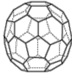
Truncated Icosahedron
