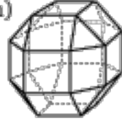
Rhombicuboctahedron
