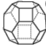
Truncated Octahedron
